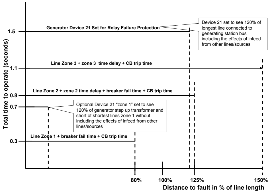
Figure 3.1.3 — Coordination Graph for Generator Trip Dependability
