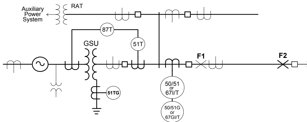
Figure 3.9.1 — Phase and Ground Backup Overcurrent Relays on Generator Step-Up Transformer
