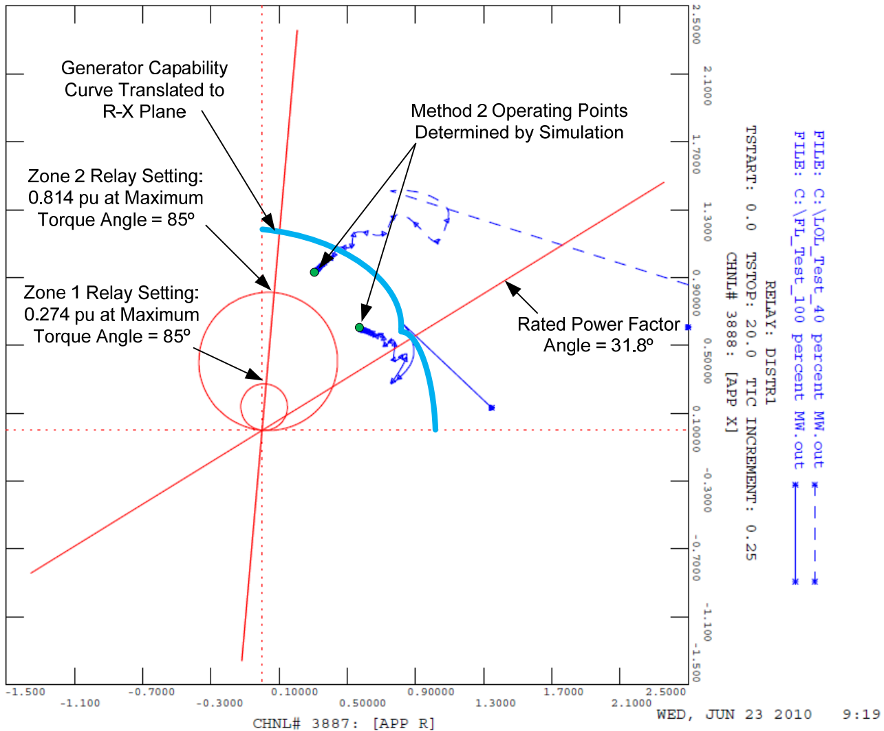
Figure 3.1.6- — Simulated Apparent Impedance Plotted against Zone 1 and Zone 2 Functions set to Coordinate with the Generator Reactive Capability Curve and Dynamic Reactive Capability During Field-Forcing
