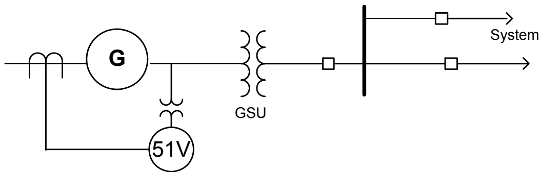
Figure 3.10.1 — Application of 51V System Backup Relays – Unit Generator-Transformer Arrangement
