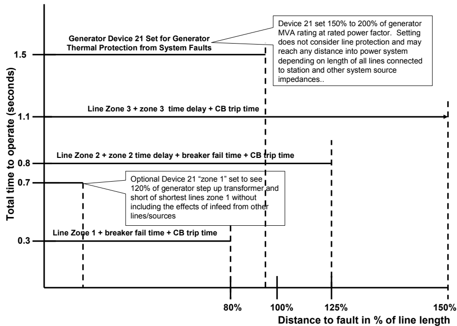
Figure 3.1.2 —Time Coordination Graph for Generator Thermal Backup Protection
