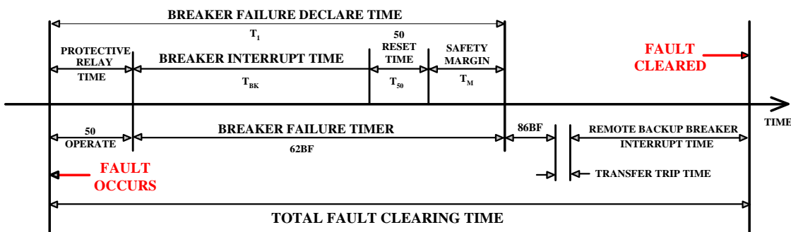
Figure 3.8.3 — Example of Breaker Failure Timing Chart 3
