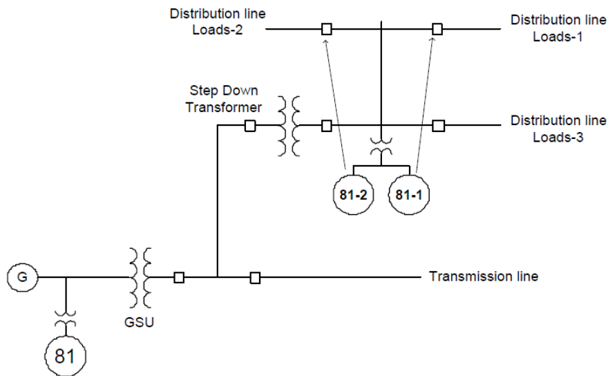
Figure 3.14.1 — Typical Location of Generator Frequency Relays and Load Shedding Relays Requiring Coordination
