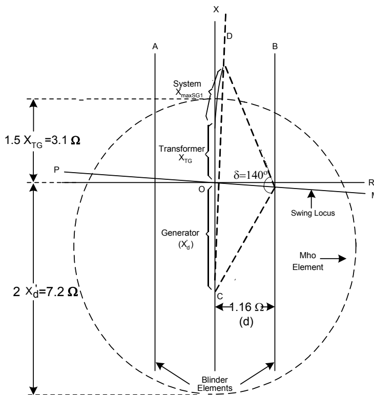
Figure 3.13.5 — Out of step relay settings
