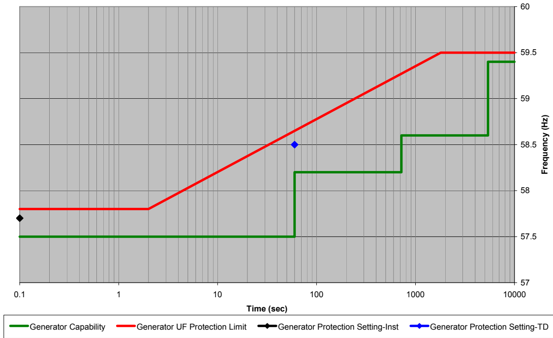
Figure 3.14.3 — Generator Underfrequency Protection Coordination Example
