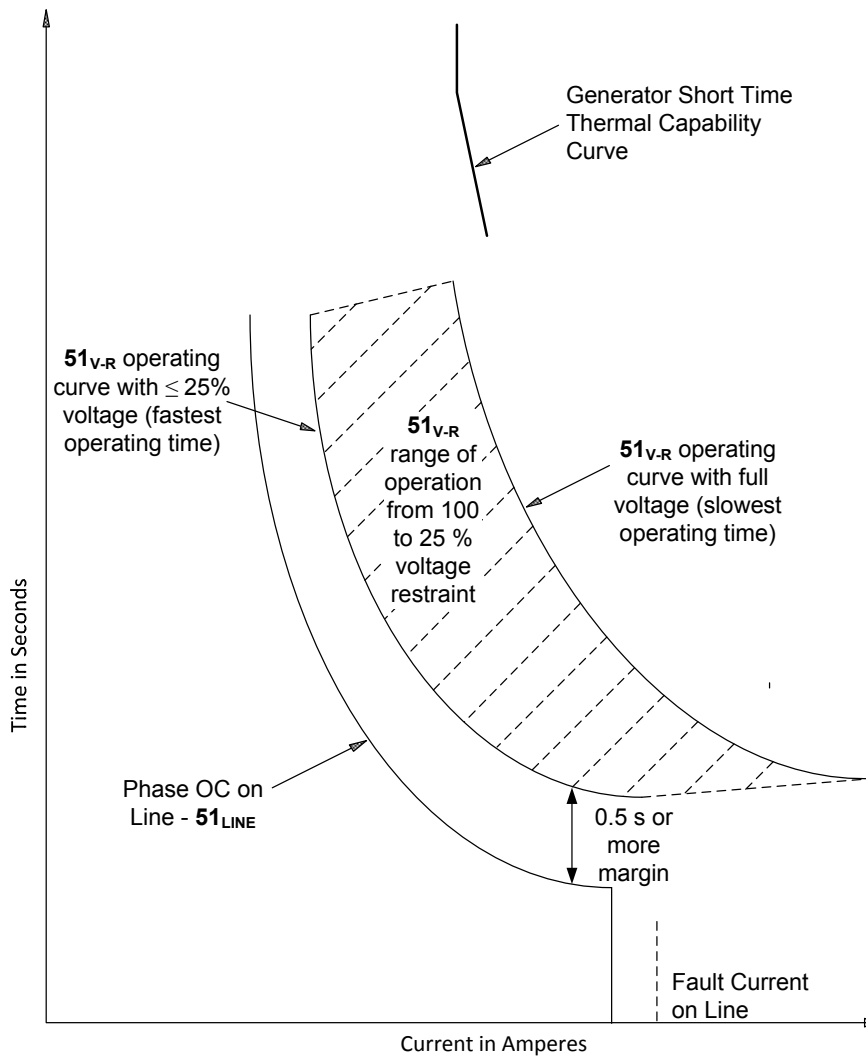
Figure 3.10.5 — Proper Coordination
