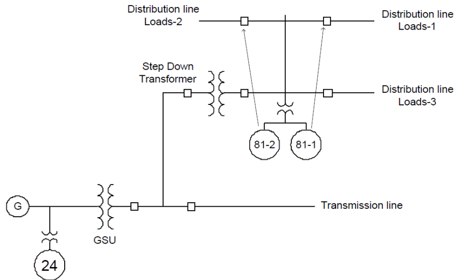
Figure 3.2.2 — Example Location of UFLS Program Relays and Generator Function 24
