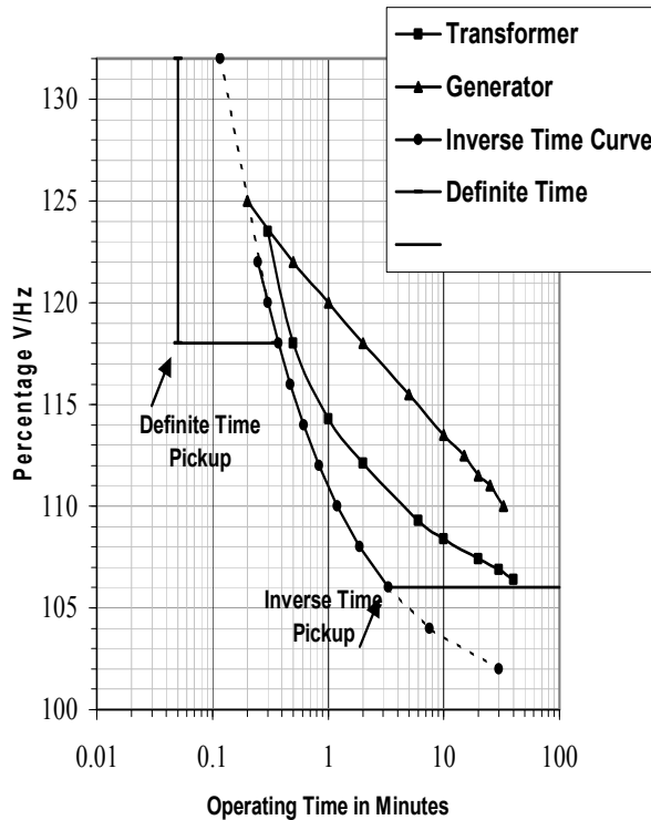
Figure 3.2.3 — Setting Example with Inverse and Definite Time V/Hz Relays
