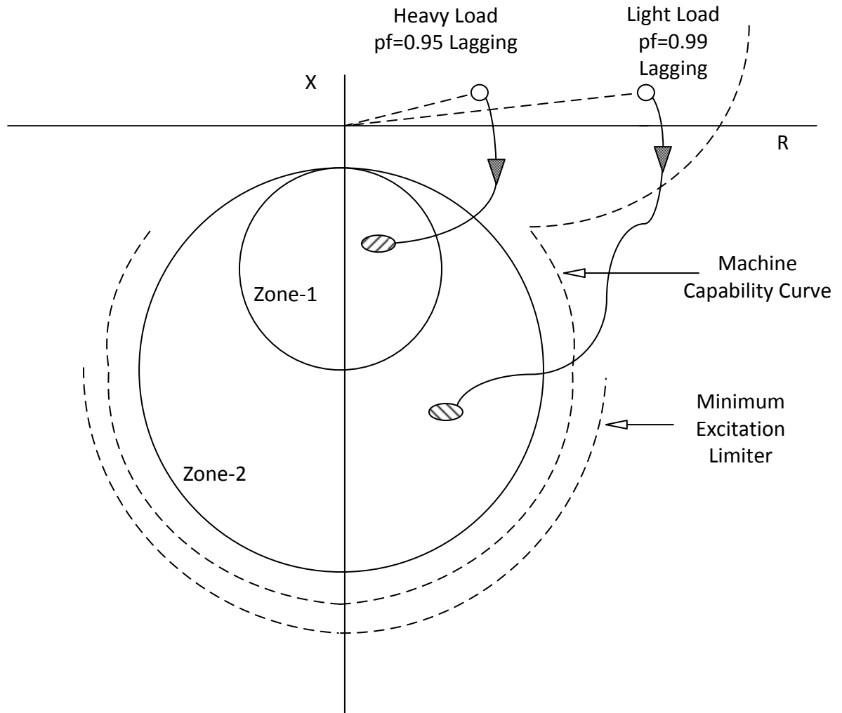
Figure 3.5.1 — (1) Locus of Swing Impedance during Light and Heavy Loads for Loss-of-Field, and (2) Relationship between Minimum Excitation Limiter (MEL) or Underexcitation Limiter (UEL)
