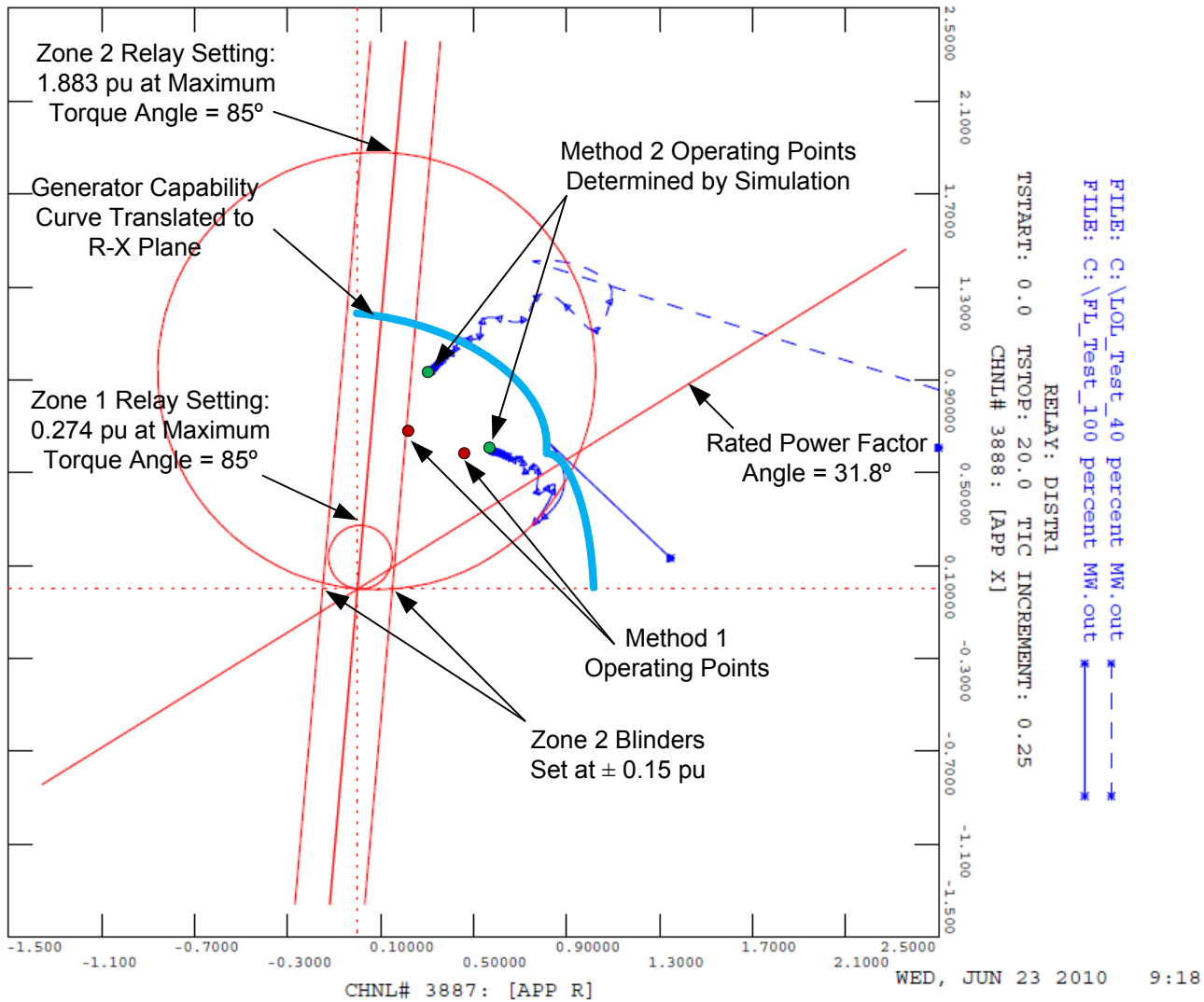
Figure 3.1.5- — Simulated Apparent Impedance Plotted against Zone 1 and Zone 2 Function with Blinders
