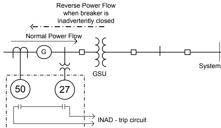
Figure 3.7.1 — Inadvertent Energizing (INAD) Protection Scheme
