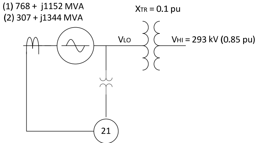
Figure E-2 — Example 1: Model of a Generator Connected to a Stressed System
