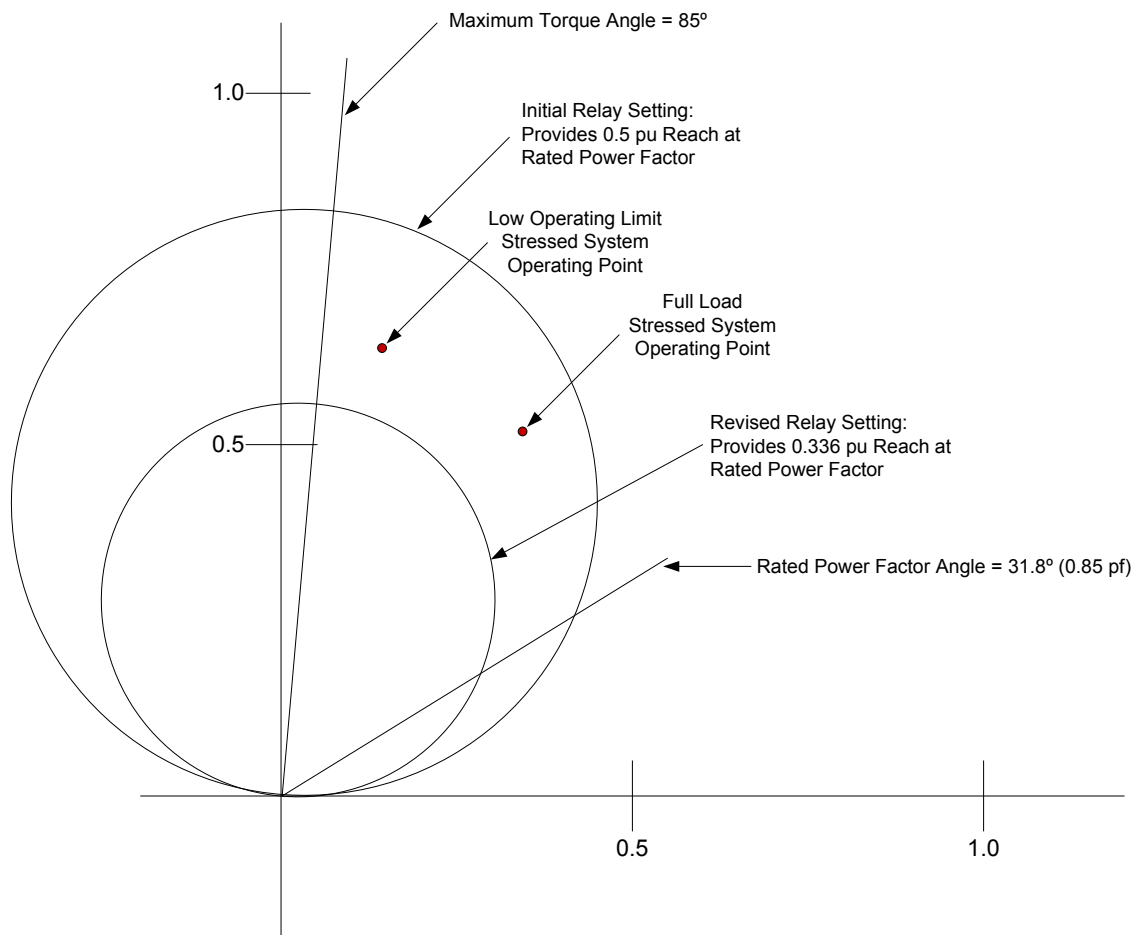
Figure E-3- — Example 1: Two Calculated Apparent Impedance Load Points Plotted against Desired and Reduced Reach Phase Distance Backup Characteristics to Meet the Restriction of the Calculated Operating Points
