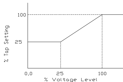
Figure 3.10.3 — Voltage Restrained OC Relay (51VR)
