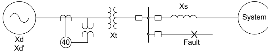
Figure 3.5.2 — Simplified System Configuration of Function 40 Relay and Fault Locations
