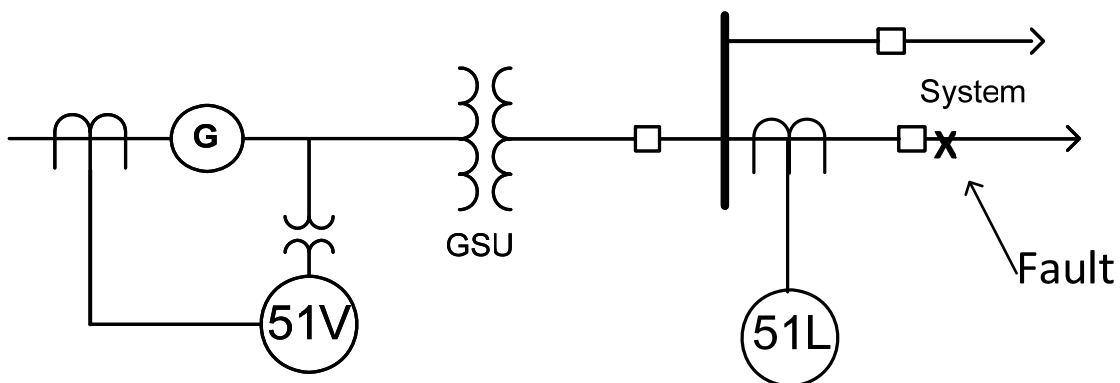
Figure 3.10.4 — System One-Line for Setting Example
