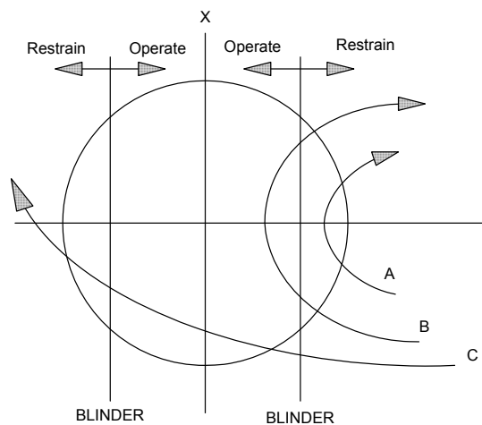
Figure 3.13.7 — “Mho”-Type Out-Of-Step Detector with a Single Blinder
