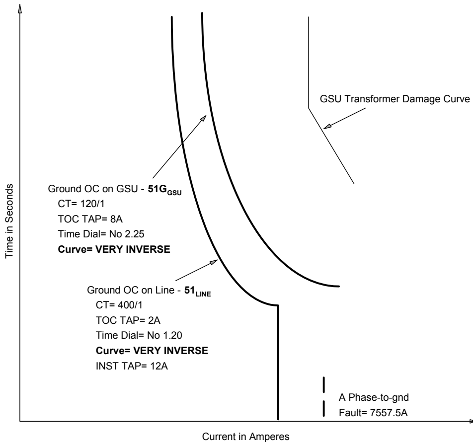
Figure 3.9.4 — Function 51TG Overcurrent Relay Characteristic Curve
