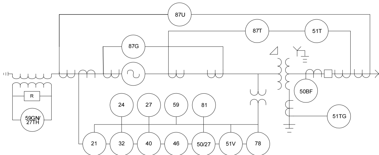
Figure 1.1 — Relay Configuration
