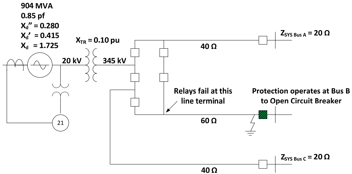
Figure 3.1.1 — 904 MVA Generator Connected to a 345-kV System by Three Lines
