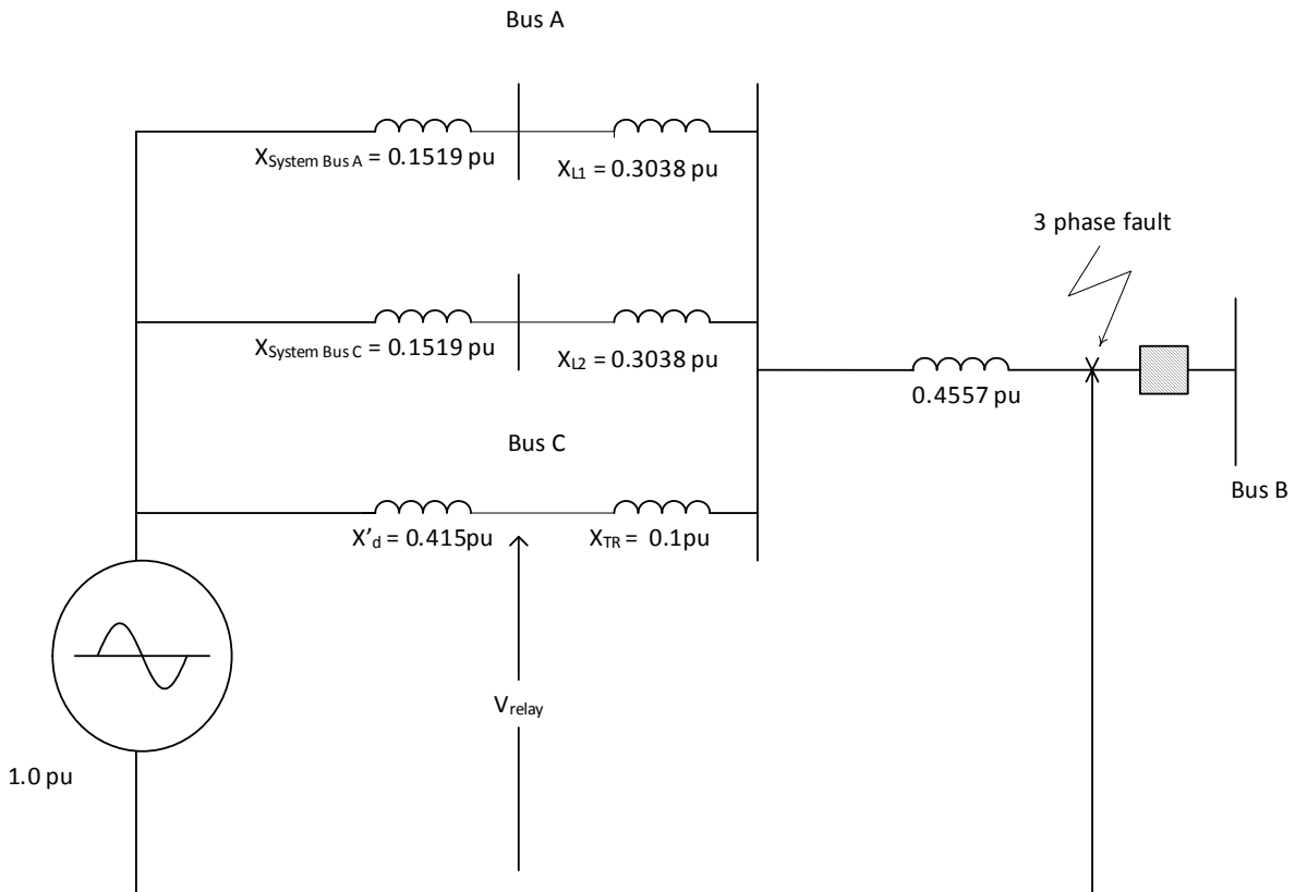
Figure E-5 — Example 2: Symmetrical Component Sequence Network
