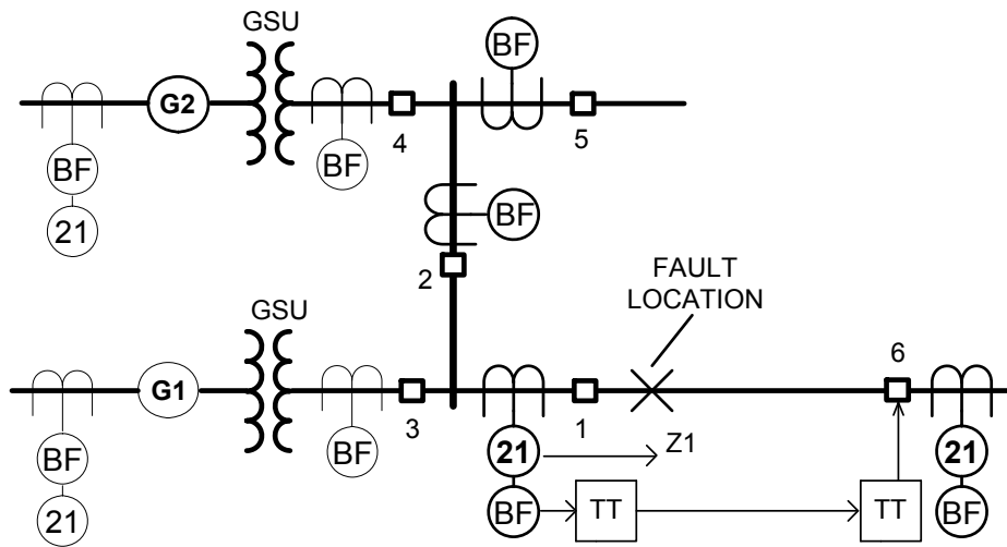
Figure 3.8.6 — Breaker Failure Coordination
