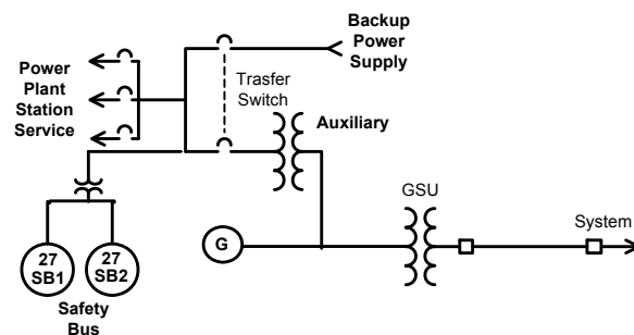
Figure 3.3.4.1 — Nuclear Power Plant Auxiliary System Power Supply
