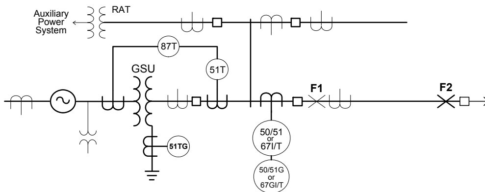
Figure 3.9.2 — Phase and Ground Backup Overcurrent Relays on Generator Step-Up Transformer
