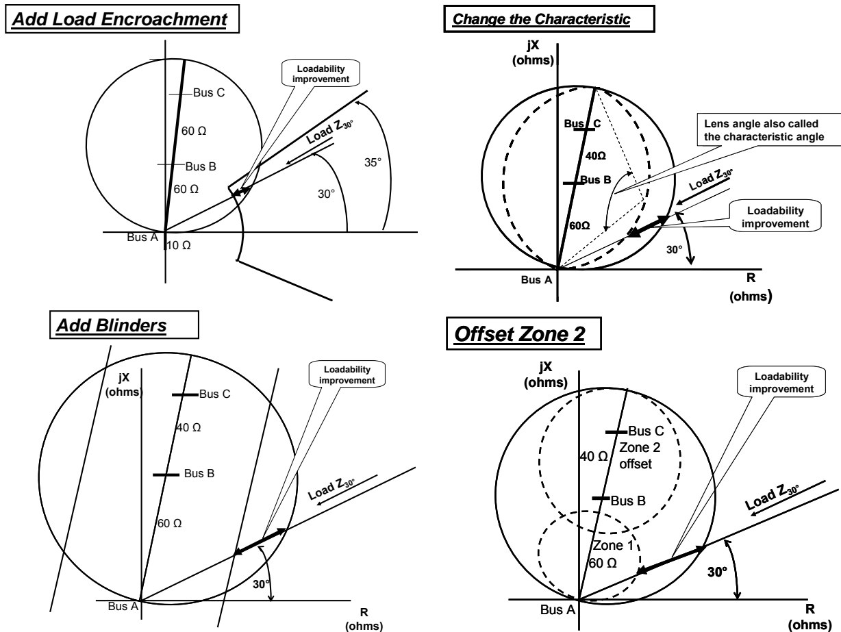
Figure 3.1.7 — Methods to Increase Loadability
