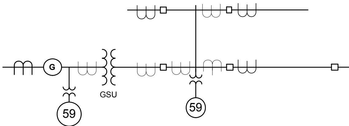
Figure 3.11.2 — Location of Overvoltage Relays Requiring Coordination
