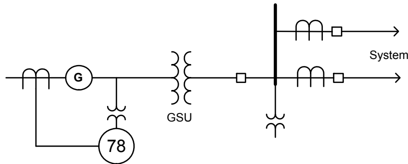
Figure 3.13.2 — Generator Out-of-Step Relay Connection
