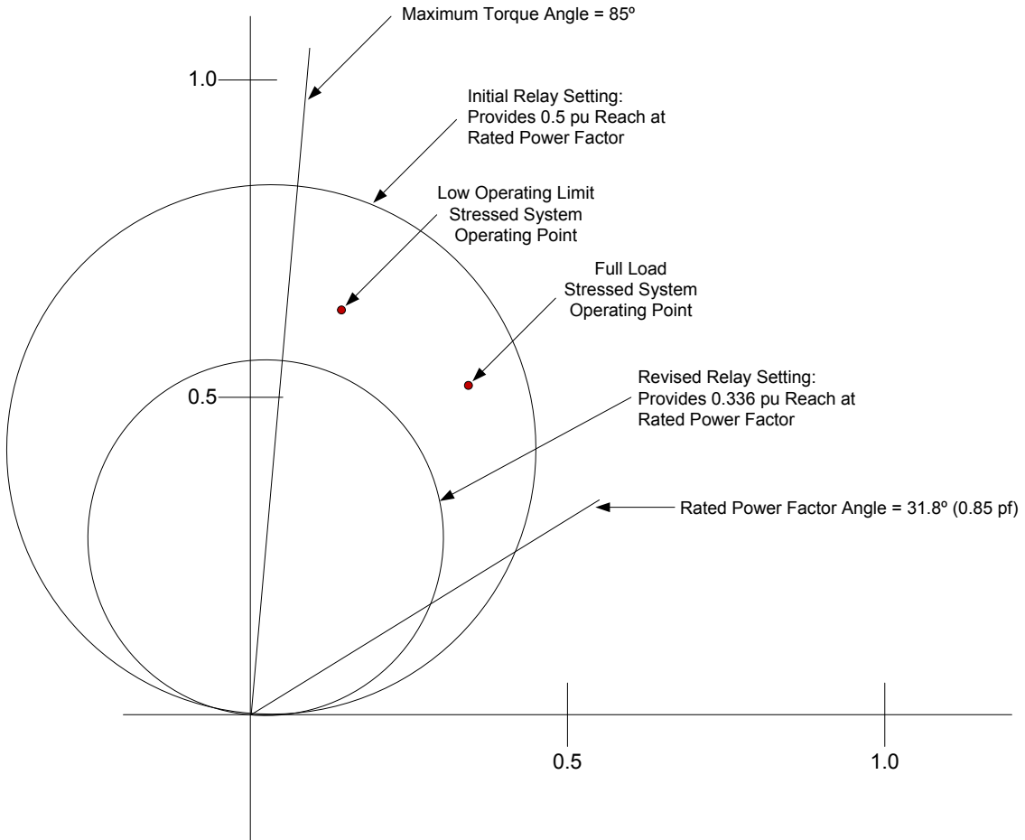
Figure 3.1.4 — Calculated Apparent Impedance versus Two Phase Distance Settings Based on 200% and 298% of Rated Generator MVA at Rated Power Factor
