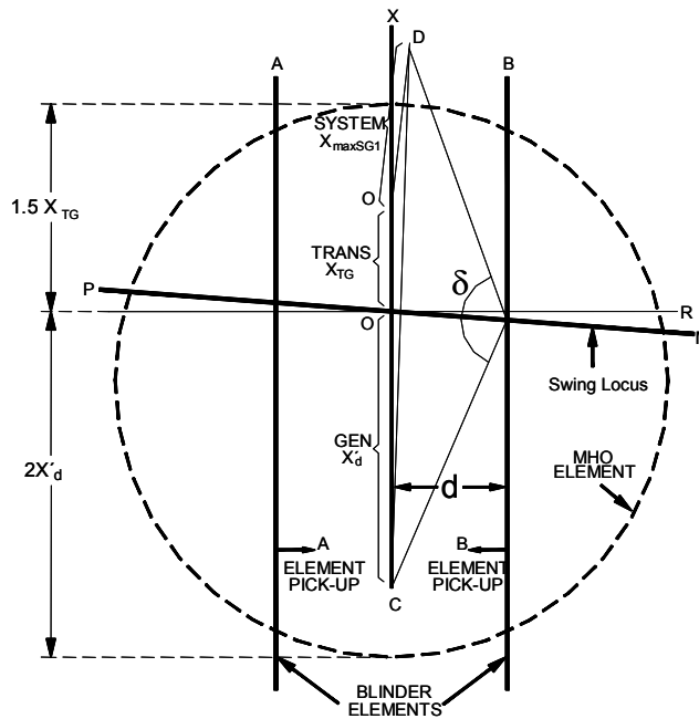
Figure 3.13.3 — Out-of-Step Protection Characteristic Using a Single Blinder Scheme
