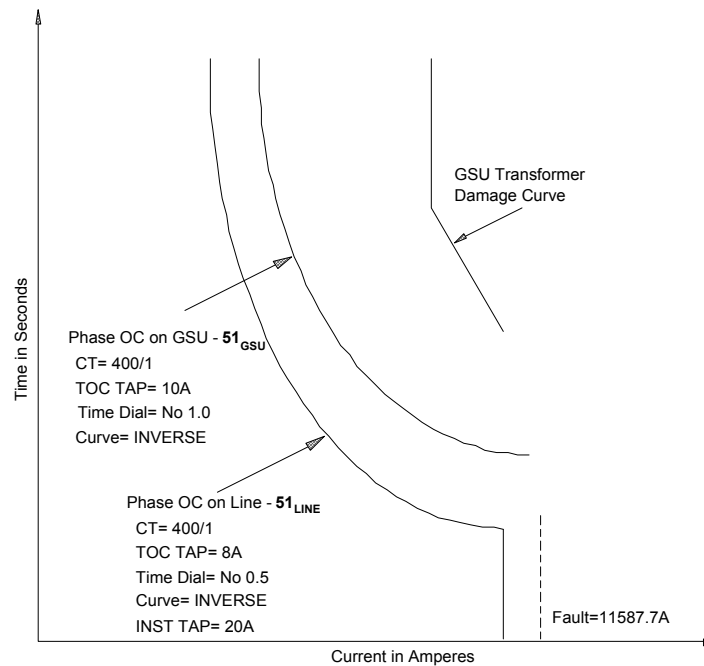
Figure 3.9.3 — Function 51TGenerator Step-Up Transformer and 51LINE (G or N) Overcurrent Relay Coordination Curves
