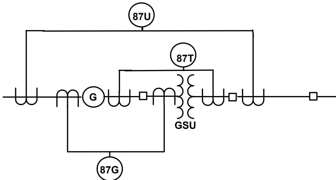
Figure 3.15.2 — Overall Differential, Transformer Differential, and Generator Differential Relays with Unit Circuit Breaker
